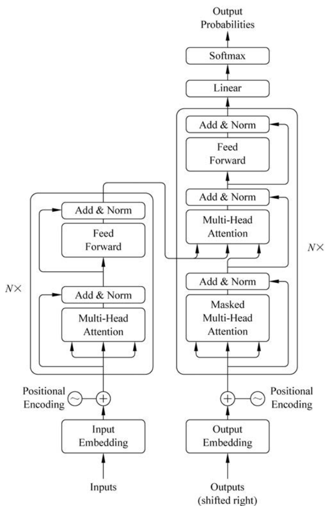
图 5-10 Multi-Head Attention
